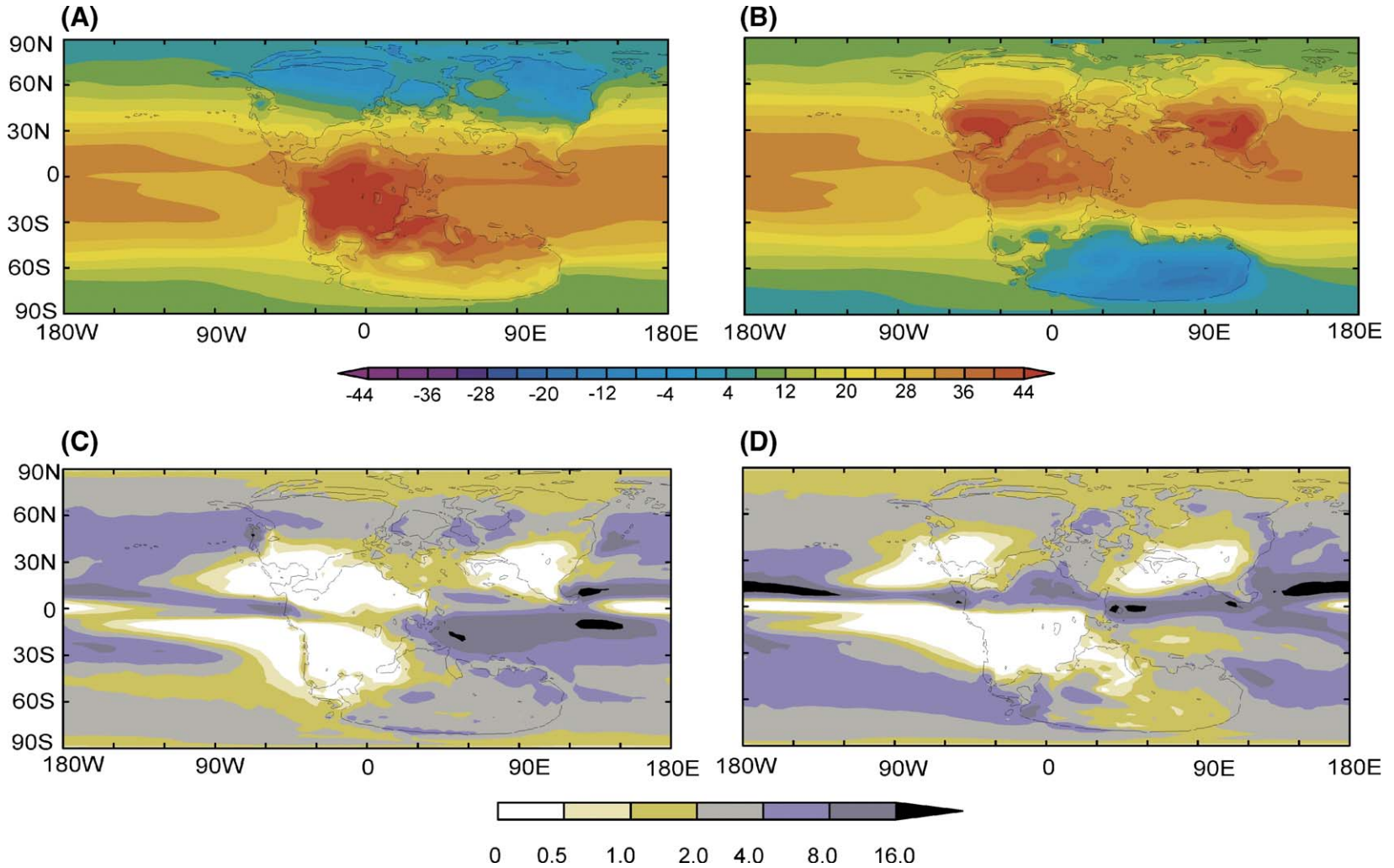
Fig. 3. (A and B) Model simulated mean seasonal temperatures for the Late Jurassic, for (A) December–January–February season and (B) June–July–August season. Units are in °C and the contour interval is every 4 °C. (C and D) Model simulated, mean seasonal precipitation for the Late Triassic, for (C) December–January–February season and (D) June–July–August season. Units are in mm/day and the contour interval is not regular.
